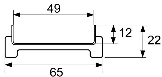
TILE INSERT - SIDE VIEW
